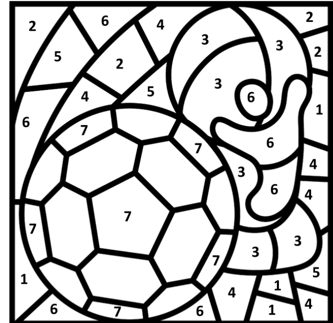
Coloring a Soccer Based on an Algorithm
