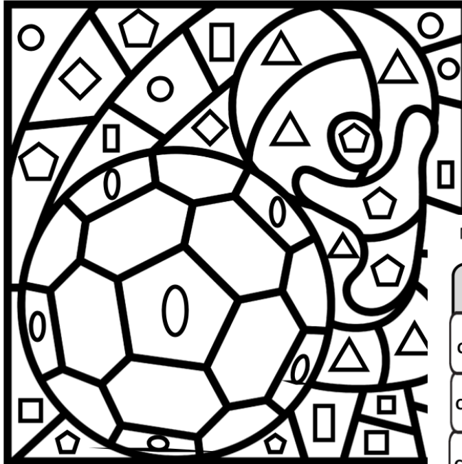
Coloring a Soccer Based on an Algorithm
